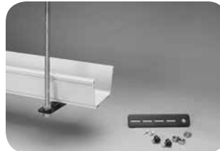
New Threaded Rod Bracket kit (FGS-HNTR-XX shown alone and attached to threaded rod)
