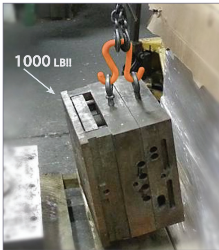
Static Load Capability Depiction for Rated Injection Molded Hooks
