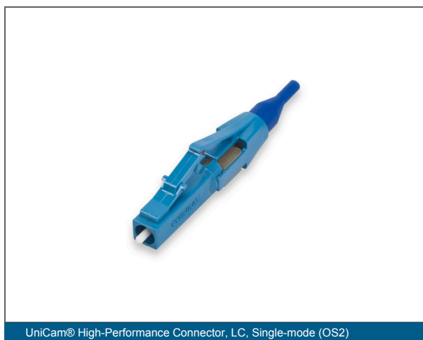
UniCam® High-Performance Connector, LC, Single-mode (OS2)
