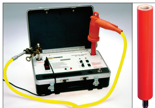
Optional Elbow Adapter C4033449 (15 & 25kV) for testing temporary grounding sets fitted with a grounding elbow. PSC4032947, 35kV, Elbow Adapter.
