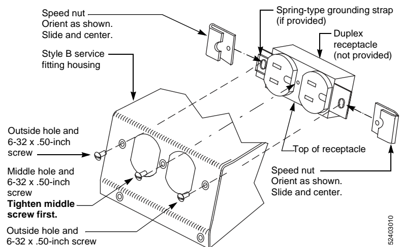
Figure 1: Service Fitting Housing and Receptacle
