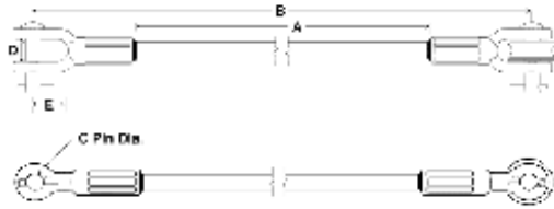
Guy Strain ; 16,000 lbs.; Clevis - Clevis - 1 Roller
