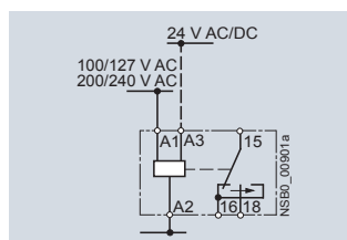
3RP2005 Passing make contact
