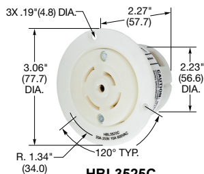
HBL3525C
