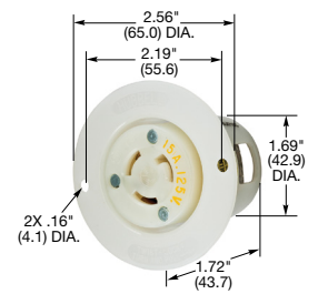
HBL4715C
