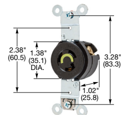
HBL4710
