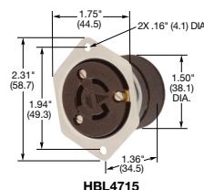
HBL4715
