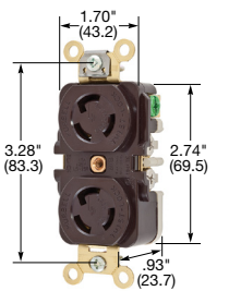
HBL4700
