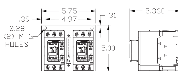
LEN00D006 (60A 6 Pole)
