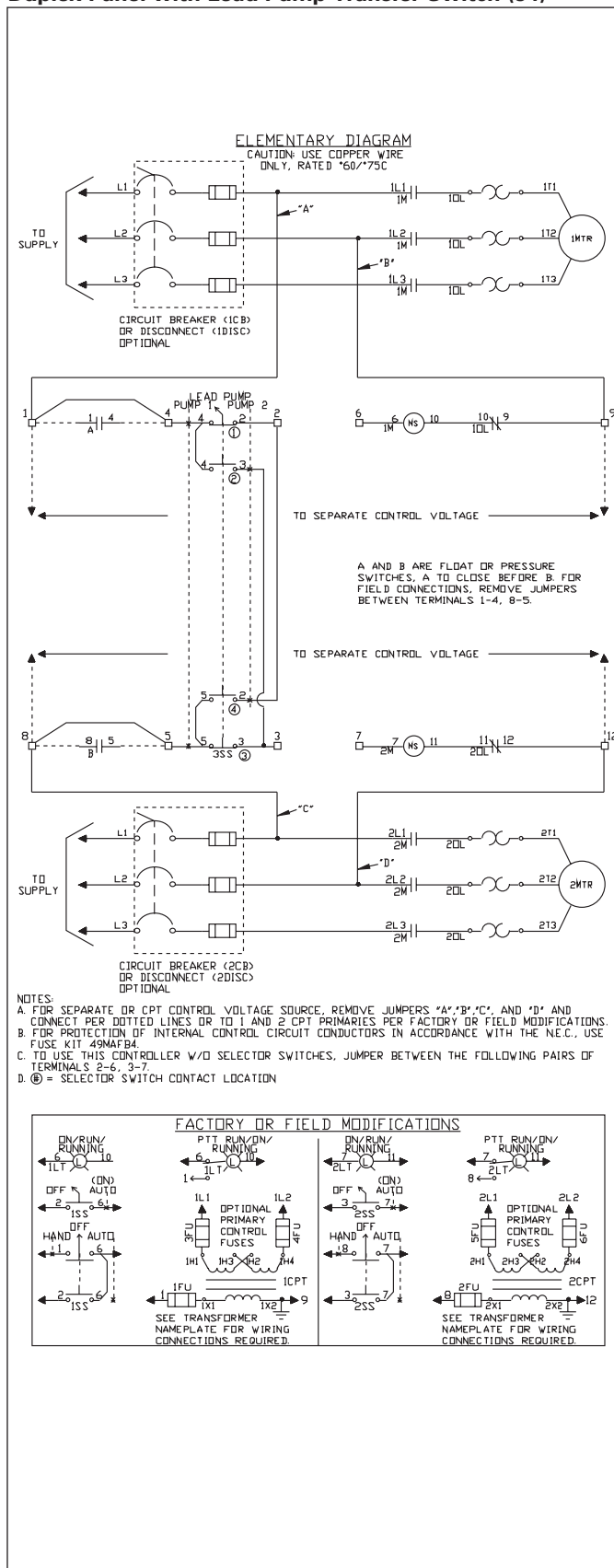
Duplex Panel with Lead Pump Transfer Switch (94)
