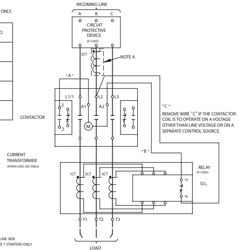
Solid State Overload 3-Phase Sizes 5-8
