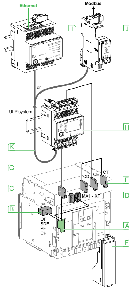
Drawout Masterpact NT/NW, PowerPact P/R Circuit Breaker
