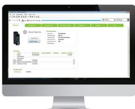
SoMove software
