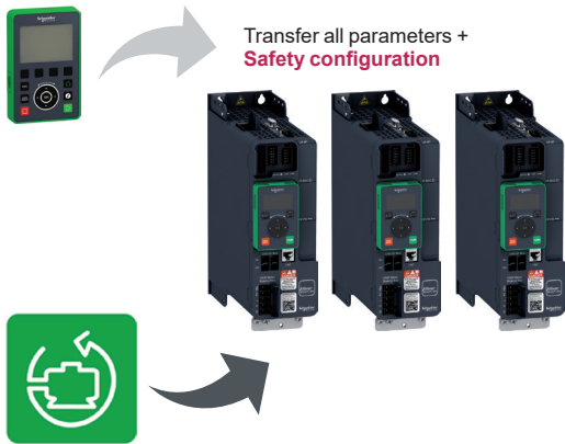
SoMove software
