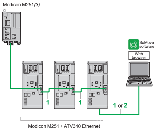
Modicon M251 + ATV340 Ethernet Example of connection on an EtherNet/IP network
