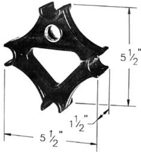
Polyethylene Spacer, 4 conductor
