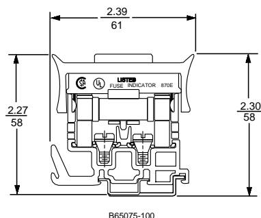
GF6, with blown fuse indicator
