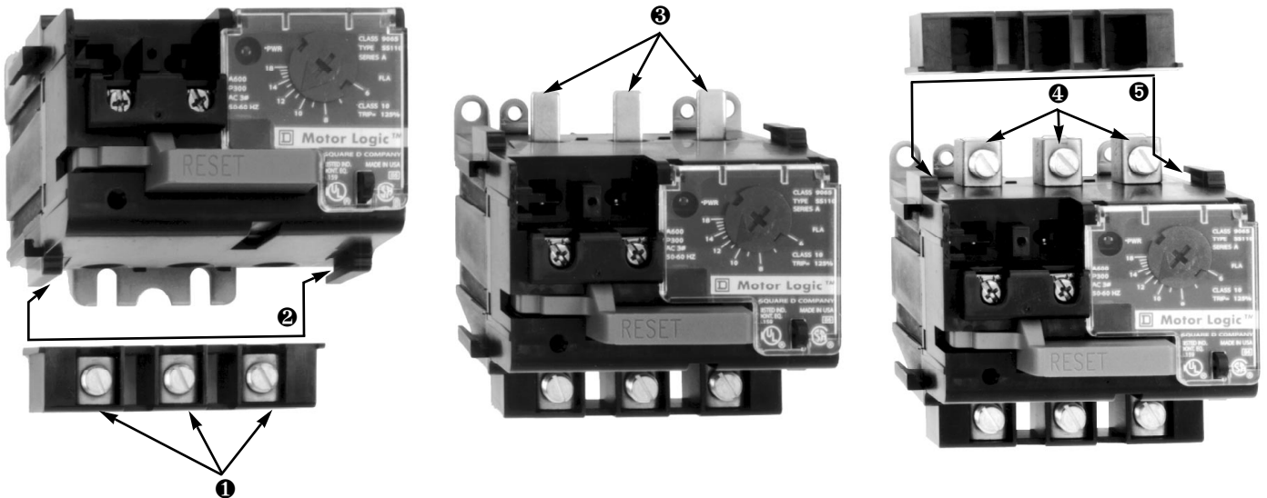
Figure 2 Assembling Lug-Lug Kit
