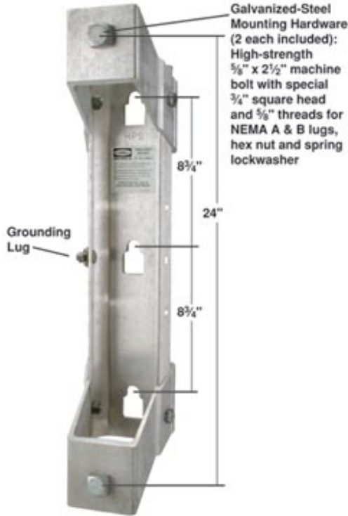
Bracket, Transformer, Wing-Rack Type
