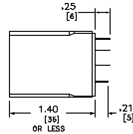
RIGHT VIEW
