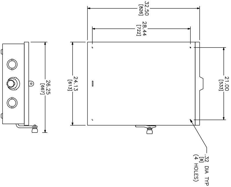
NEMA TYPE 3R ILLUSTRATED
