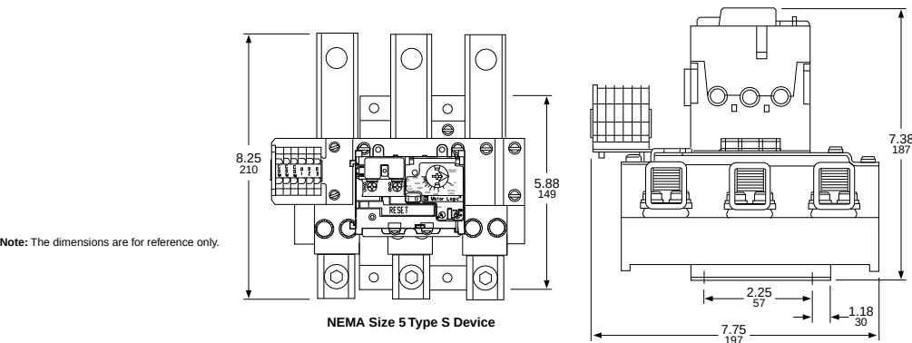
Figure 16 - NEMA Size 5 Type S Device
