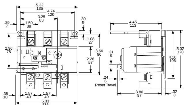
Figure 15 - Size 4 Devices
