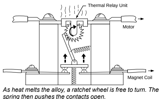
Figure 2 - Operation of the Melting Alloy Overload Relay
