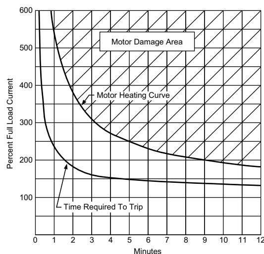
Figure 5 - Overload Relay Trip Curve
