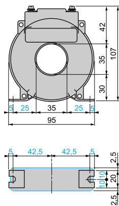
Figure 26 - LT6CT Current Transformer
