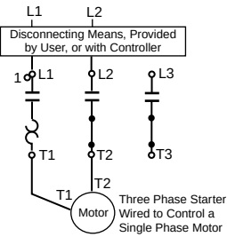
Figure 10 - Jumper Strap Kit Diagram
