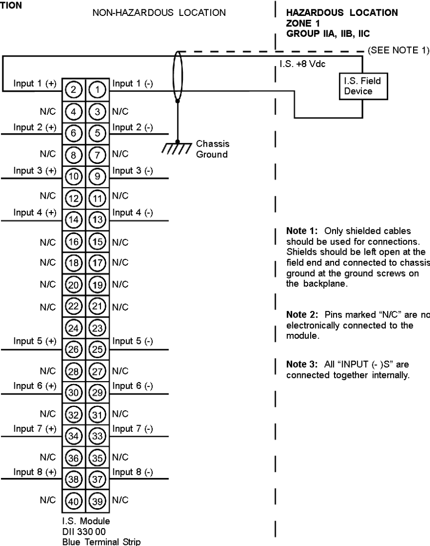
31001365 Rev 00 140 DII 330 00 Wiring Diagram
