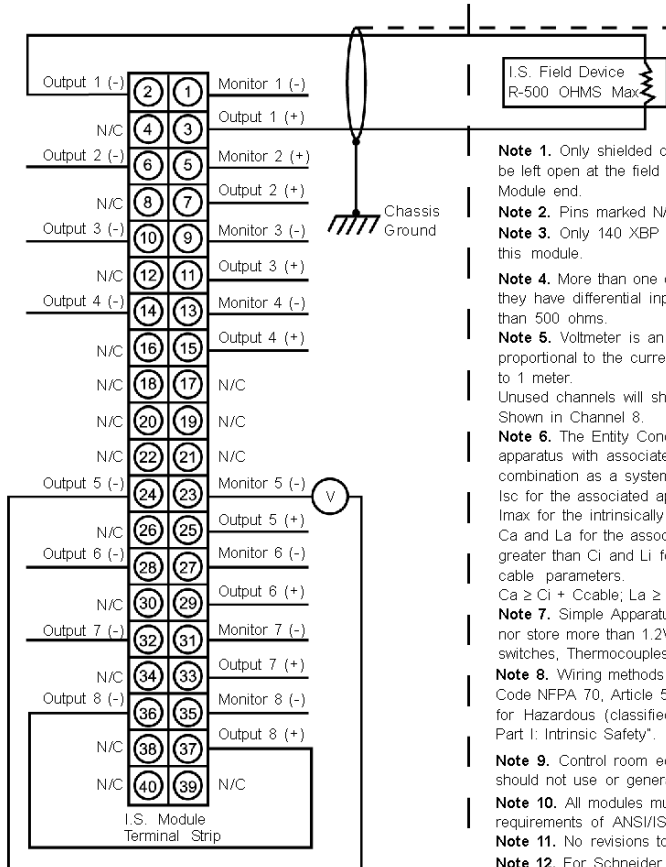
140 AIO 330 00 Wiring Diagram 31001364 Rev 01
