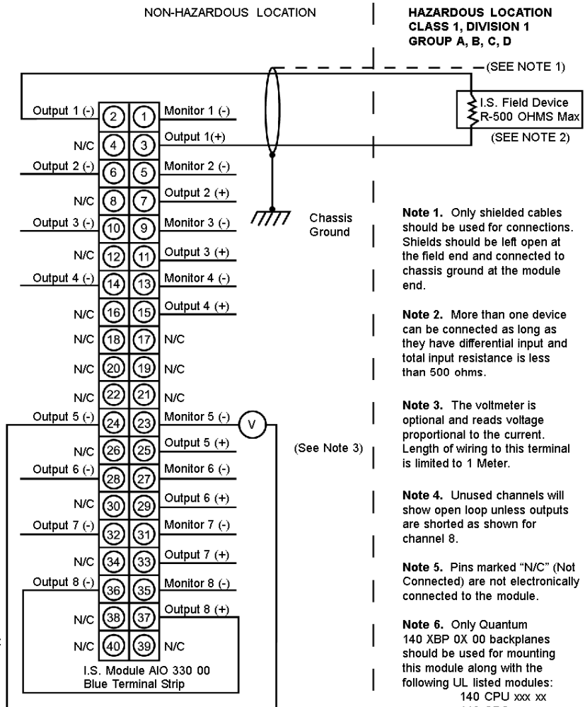
31001364 Rev 00 140 AIO 330 00 Wiring Diagram
