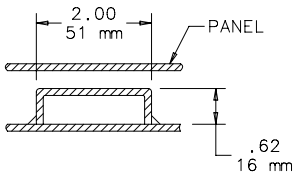
SECTION Z-Z
