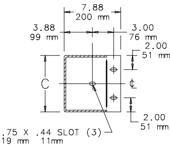
SECTION W-W
