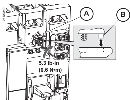
M-frame Manually-Operated Circuit Breakers
