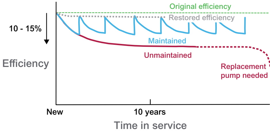
Average wear trends for maintained and unmaintained pumps (courtesy of ETSU – Energy Savings in Industrial Water Pumping Systems).
