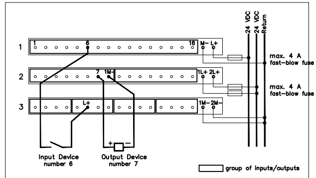
Wiring for 2-wire field device
