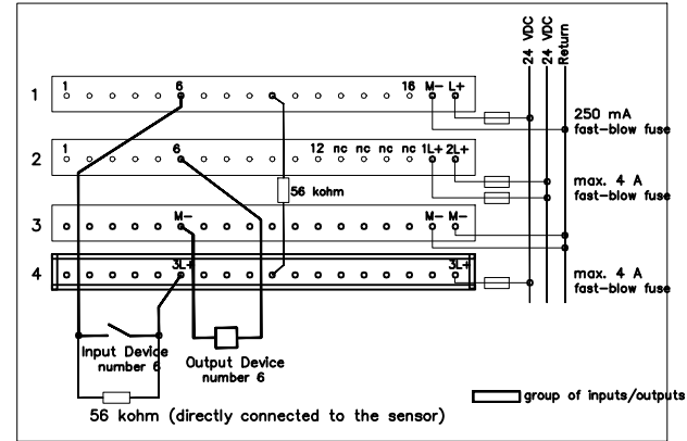
Wiring for 2-wire field device
