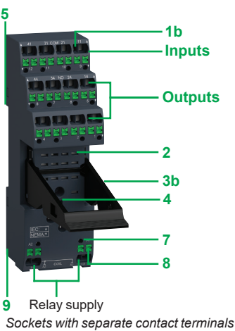
Sockets with separate contact terminals
