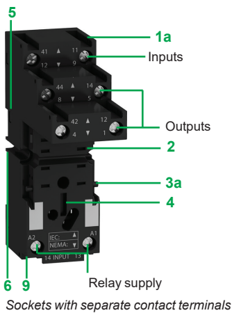
Sockets with separate contact terminals
