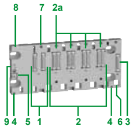
BMEXBP0400/0800 backplanes
