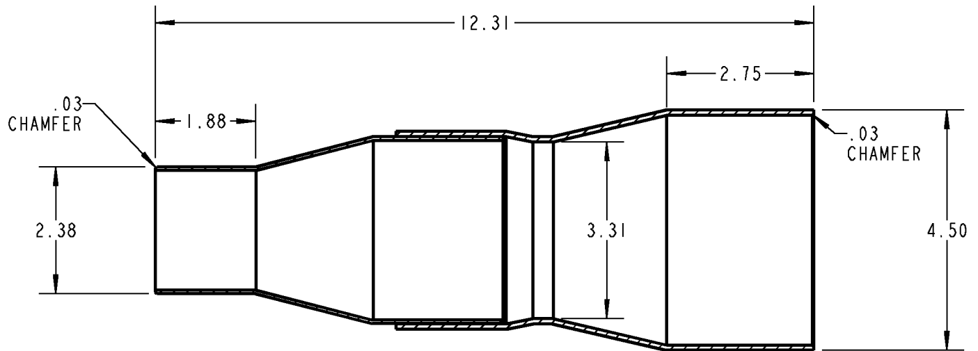
E252NJS 4" x 2" REDUCER
