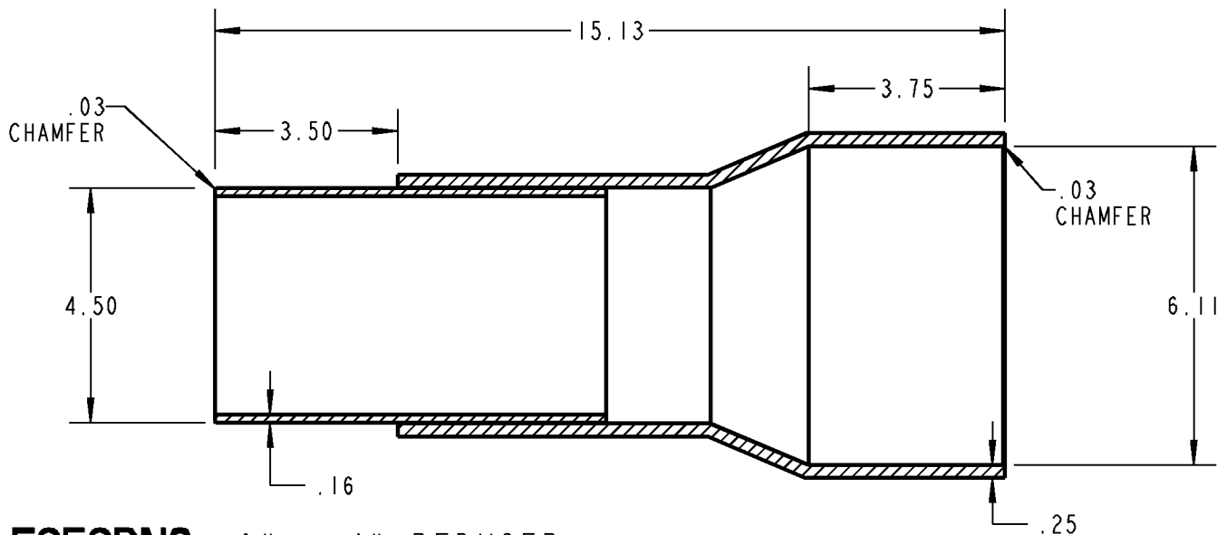
E252RNS 6" x 4" REDUCER
