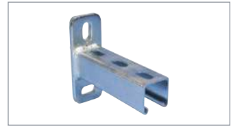
Strut Cantilever Arm Type A, Slotted KA25H#####EG
