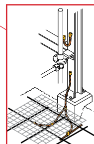
Prefabricated Mesh for Switch Shaft and Operating Handle Grounding
