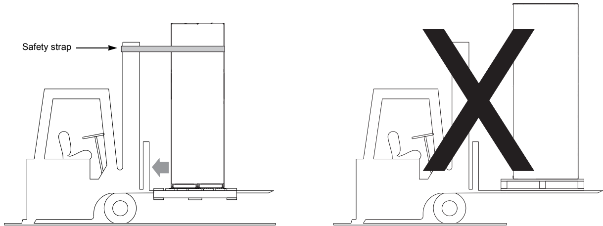
Figure 1: Handling with a Forklift
