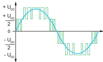
ATV600 with 3-level technology
