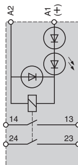
2 N/O
