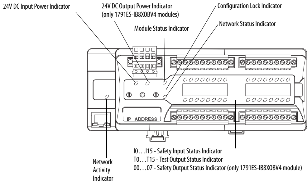
Figure 23 - 1791ES Module Status Indicators
