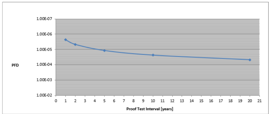
Figure 30 - PFD vs. Proof Test Interval 1732ES-IB12X0BV2, 1732ES-IB12X0B4, 1732ES-IB8X0BV4, 1732ES-IB8X0B8, 1732ES-IB16 - Dual Channel Inputs
