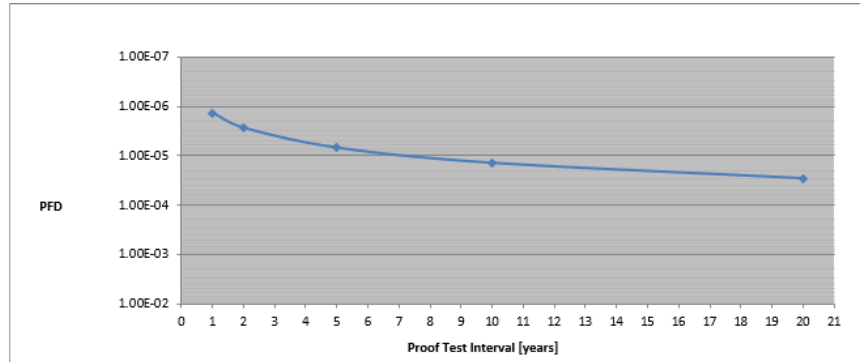
Figure 26 - PFD vs. Proof Test Interval 1791ES-IB8XOBV4 Dual Channel Outputs
