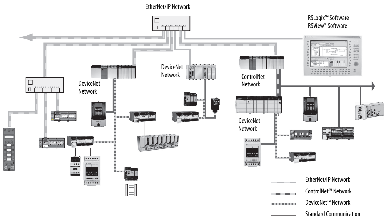
Figure 14 - Safety Interlocking and Control Via CIP Safety (linear and star topology)
