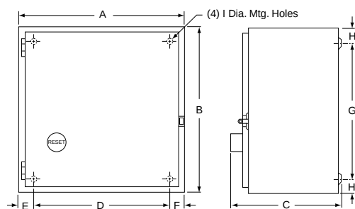
Figure 16.12: NEMA 1
