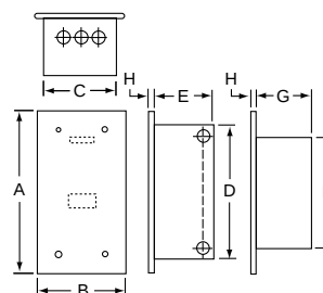
Figure 16.34: Flush Mounting General Purpose Enclosures
