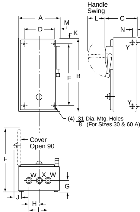
Figure 16.24: NEMA 1 Enclosure, Combination Devices
