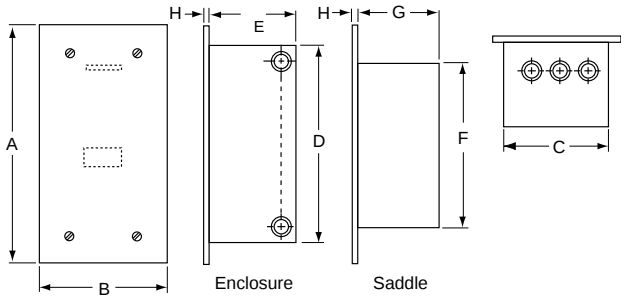
Figure 16.20: NEMA 1 Flush Mounted
