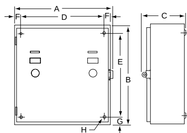
Figure 16.28: NEMA 1 Enclosure—Non-Combination
