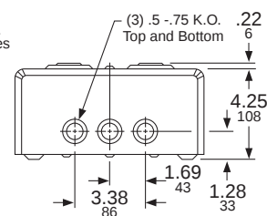
Classes 2511, 2512, Types M & T Sizes M-0 and M-1 NEMA 1 General Purpose Enclosure Approximate Shipping Weight: 9 lb
