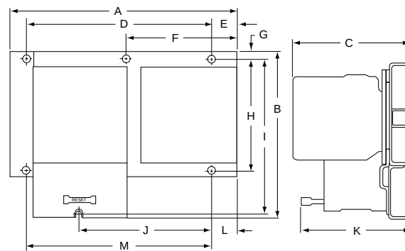
Figure 16.11: Class 8736 Starter, Open Type
