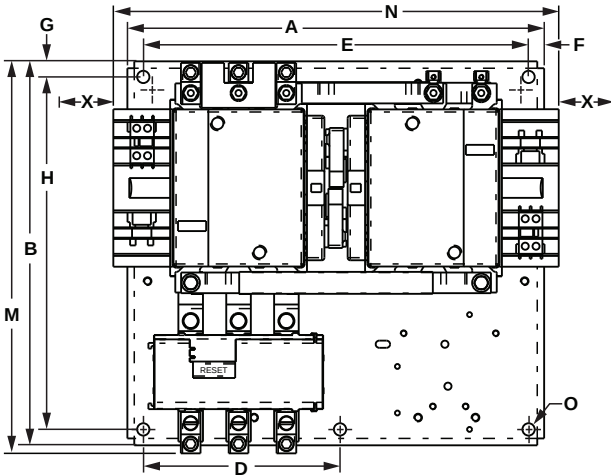
Reversing T36EN23 / T36FN23
