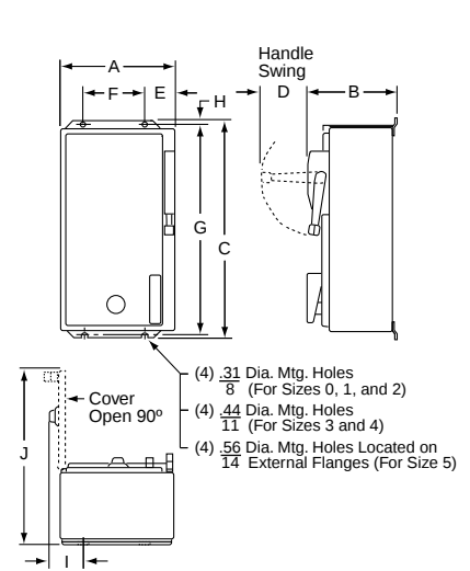
Figure 16.17: NEMA 12/3R Enclosure
