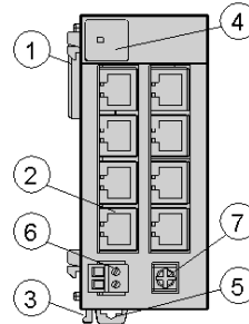
TM2ARI8LRJ module with 8 x RJ11 connectors
