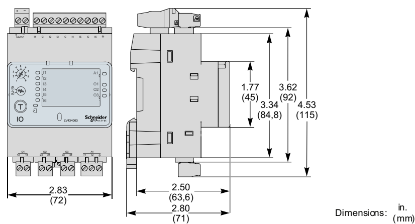
I/O (Input/Output) Application Module
