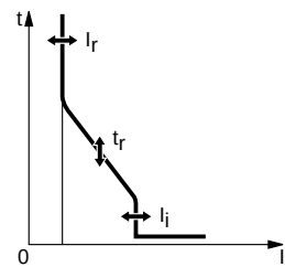
MicroLogic 2.0A and 3.0A Trip Unit Settings
