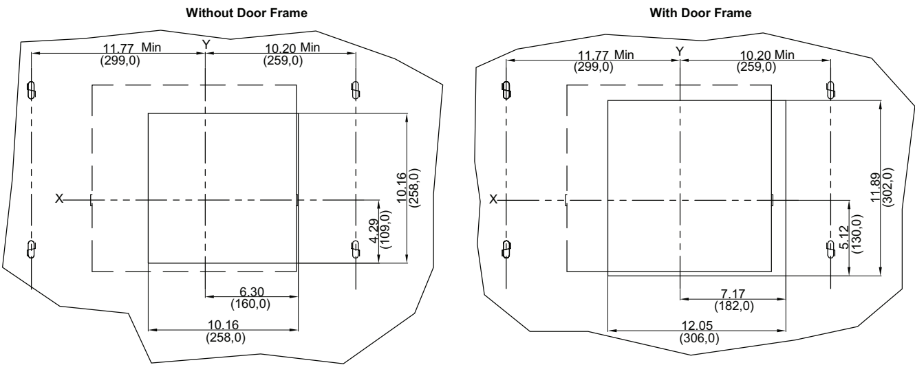
Figure 45 - 800–1200 A MasterPact NT UL/ANSI Four-Pole Drawout—Door Cutout Dimensions
