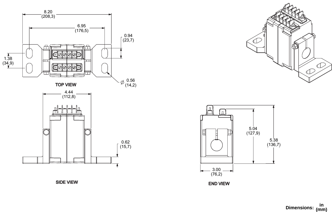
Figure 74 - 800–1600 A External Neutral Current Transformer (Switchboards and Switchgear)
