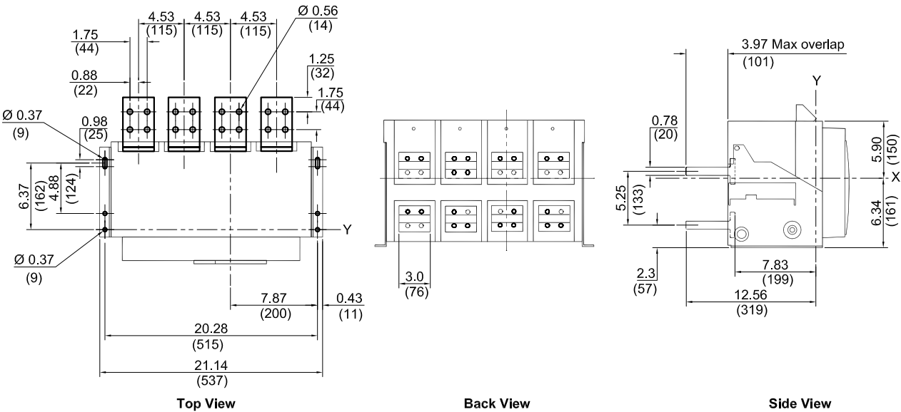
Figure 130 - 2500–3000 A Rear-Connected "T" Horizontal (RCTH)
