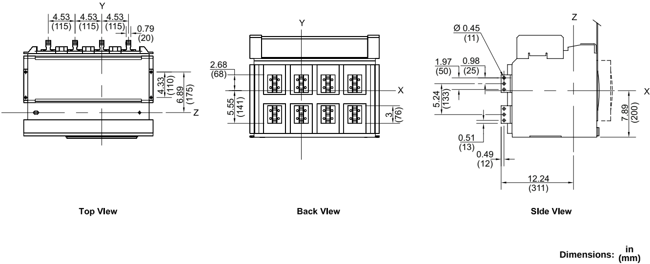
Figure 164 - 800–3200 A Rear-Connected "T" Vertical (RCTV)
