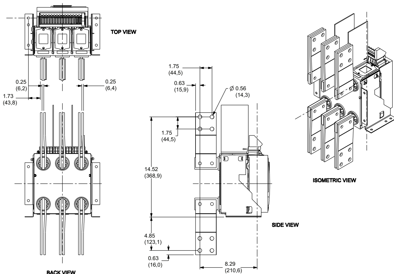
Figure 38 - 1600 A MasterPact NT UL Three-Pole Fixed—RCV Rear-Connected Vertical
