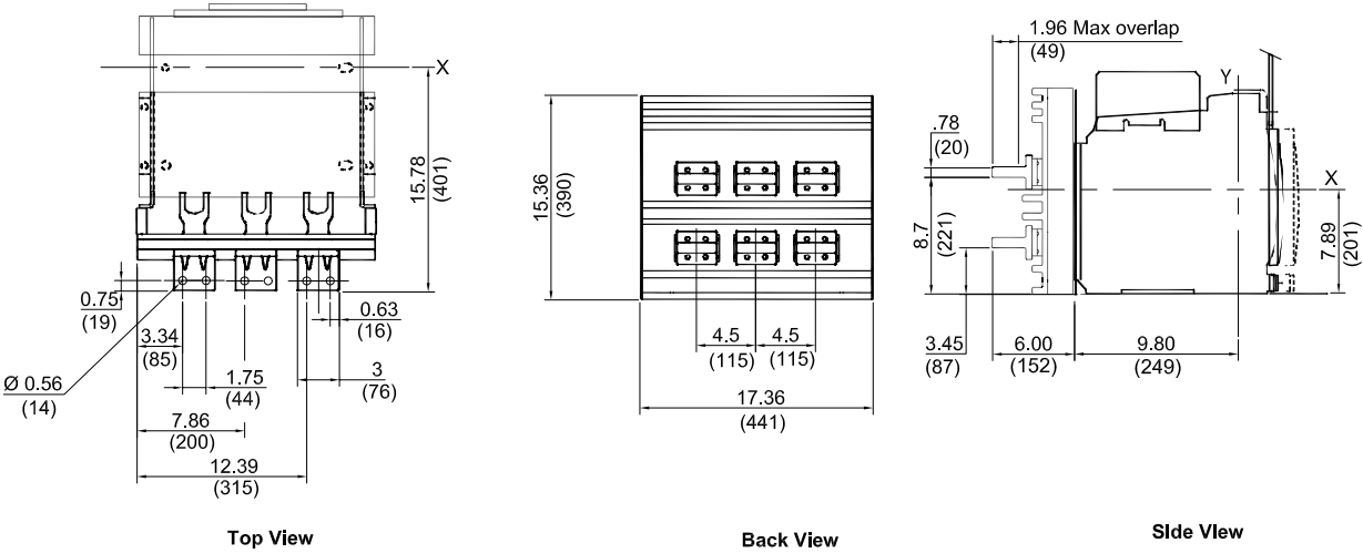
Figure 78 - 800–2000 A Rear-Connected "T" Horizontal (RCTH)
