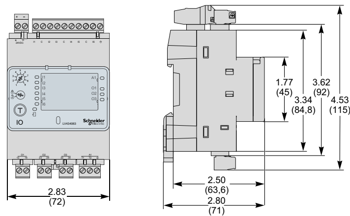
Figure 173 - IO (Input/Output) Application Module
