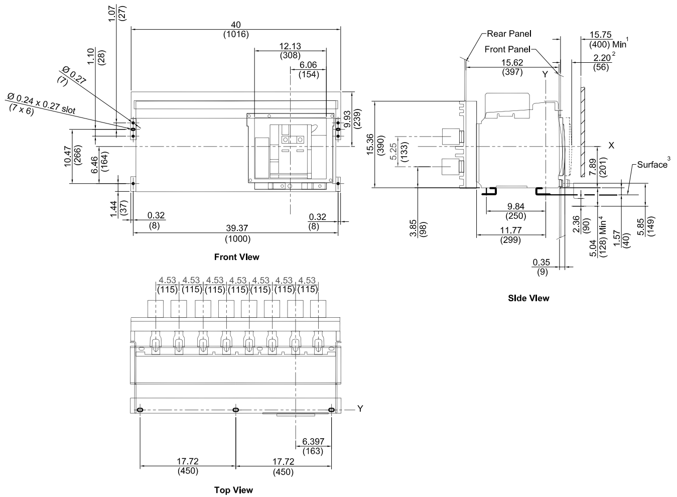
Figure 117 - 3200 A L1 and 4000–6000 A Master Drawing
