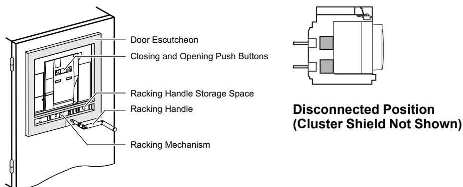
Figure 2 - Racking Handle and Mechanism
