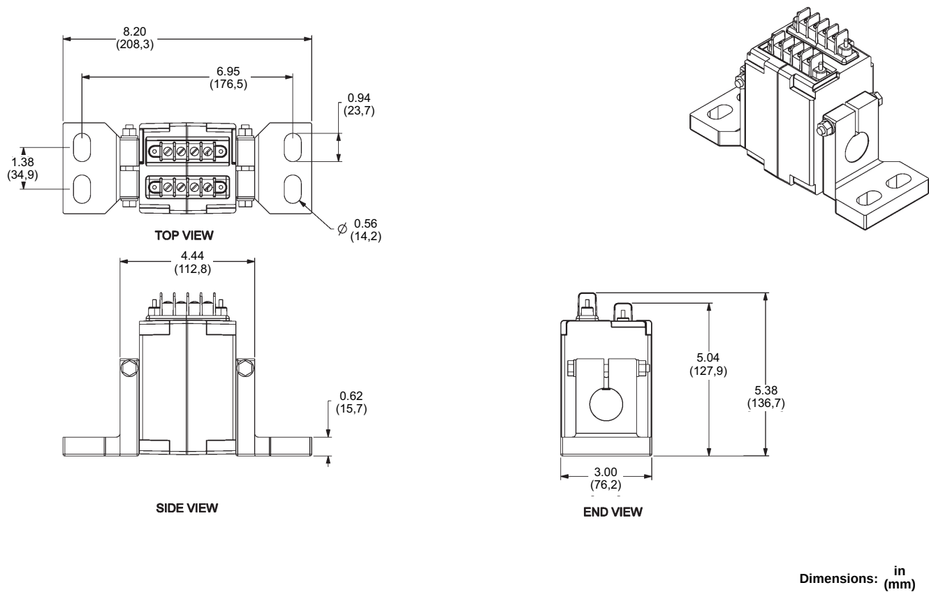
Figure 73 - 800–1600 A External Neutral Current Transformer
