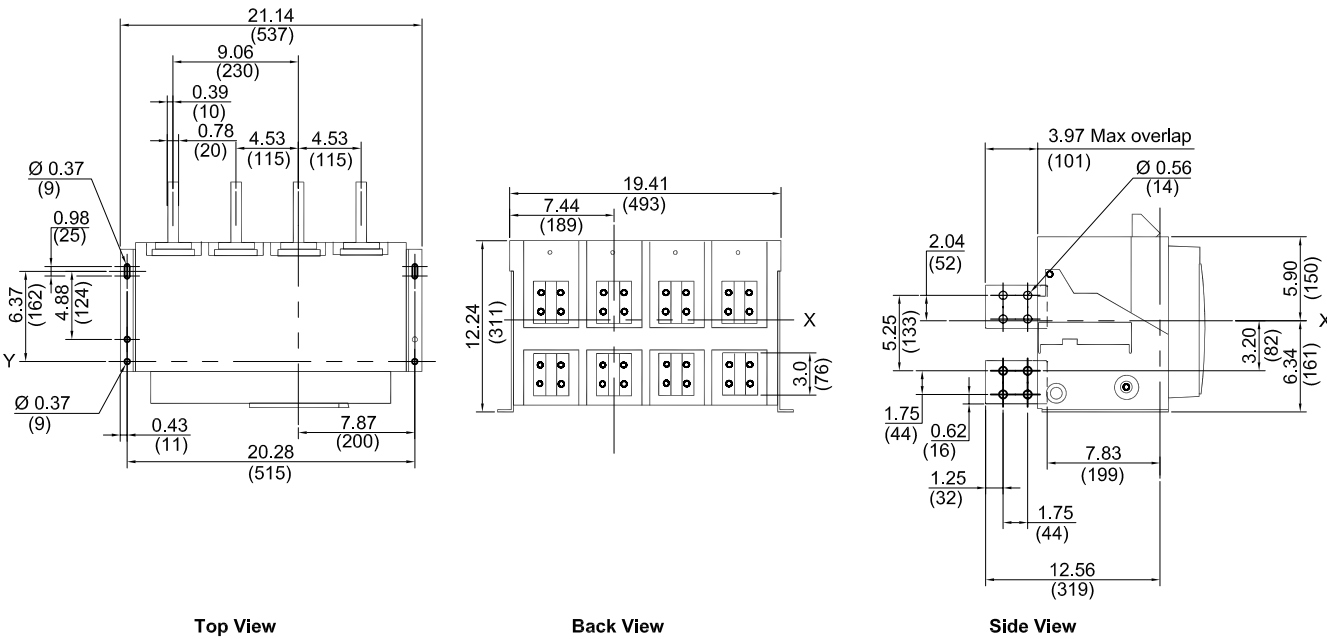
Figure 129 - 2500–3000 A Rear Vertical "T" Horizontal (RCTV)
