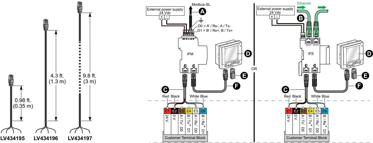
Figure 6 - FDM121 Connections
