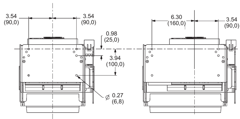
Figure 33 - 800–1200 A MasterPact NT UL/ANSI Drawout and Fixed—Pan Dimensions
