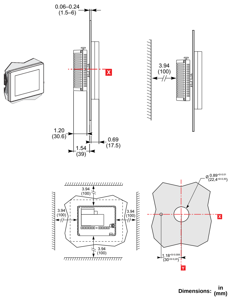
Figure 179 - FDM128 Switchboard Display Mounting on Panel
