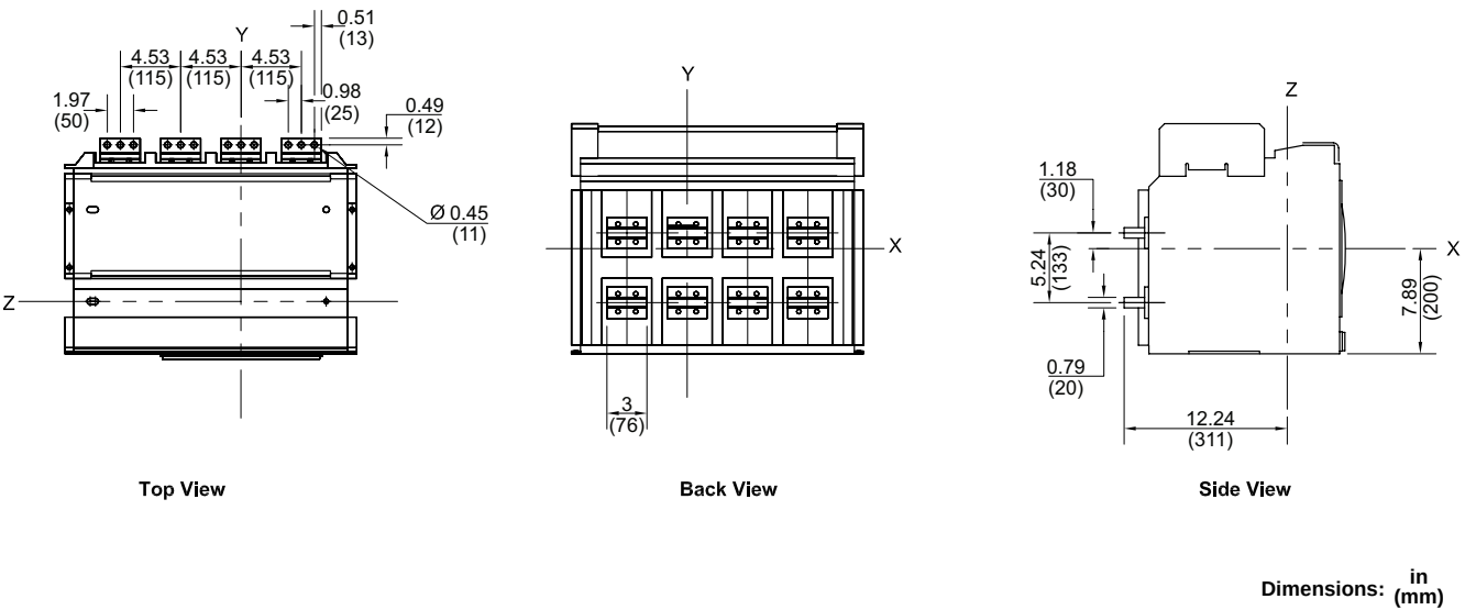
Figure 165 - 800–3200 A Rear-Connected "T" Horizontal (RCTH)
