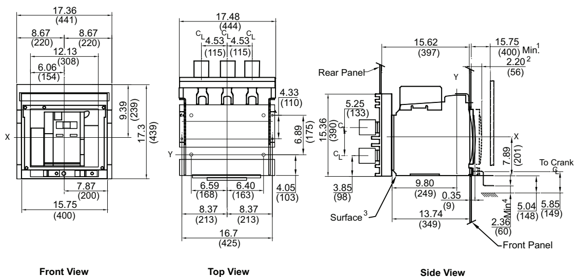
Figure 76 - 800–3000 A and 4000 A (H1, H2, H3) Master Drawing
