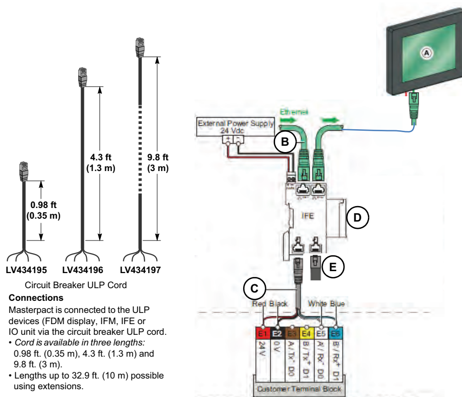
Figure 7 - FDM128 Connections
