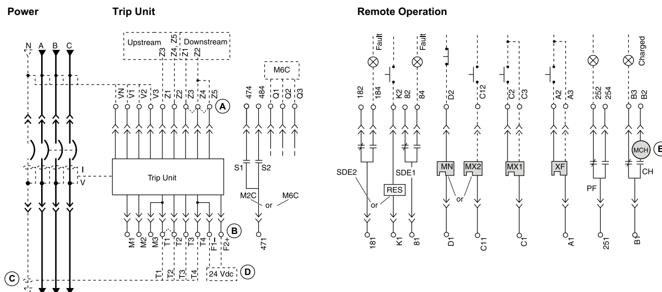
Figure 23 - Wiring Diagrams for MasterPact NW Circuit Breakers
