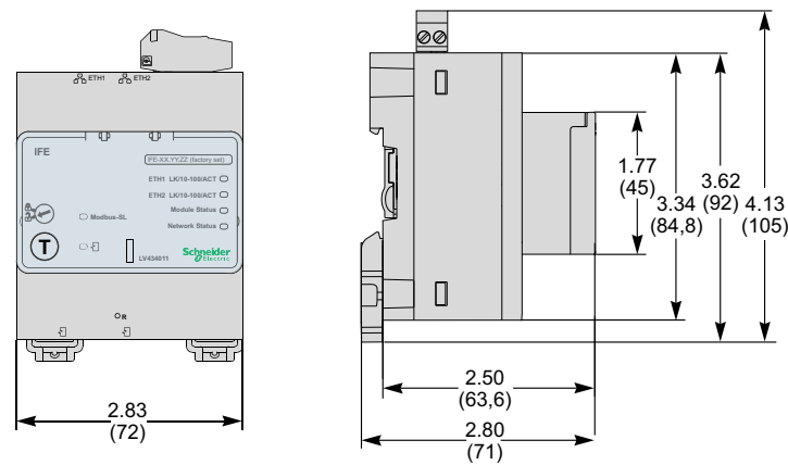
Figure 172 - IFE Ethernet Interface
