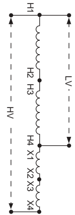
Wiring Diagram 4
