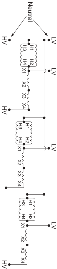
Wiring Diagram 8
