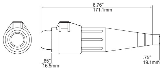
Female connector
