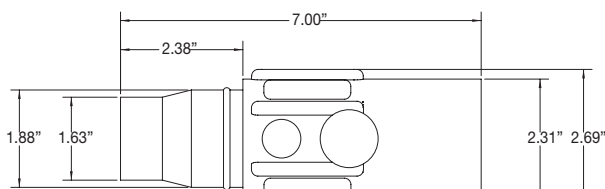
Male connector
