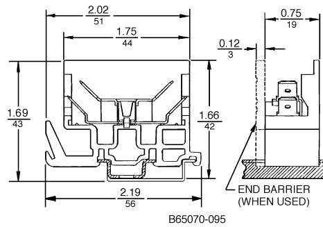
Figure 26 - Type GS6
