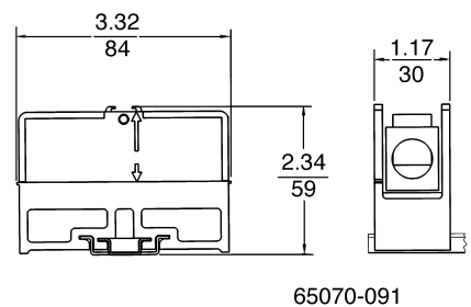
Figure 22 - Type GE6
