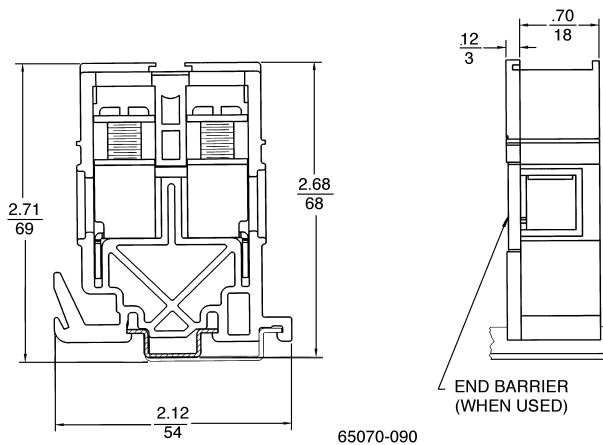
Figure 21 - Type GD6
