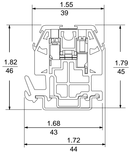
Figure 18 - Type GM6
