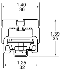
Figure 19 - Type GK6
