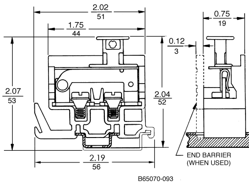
Figure 27 - Type GG6
