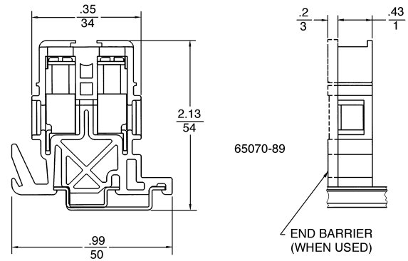
Figure 20 - Type GC6
