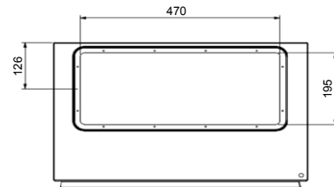
Cable entry type G: Enclosure width 600 (23.62) mm (in.).
