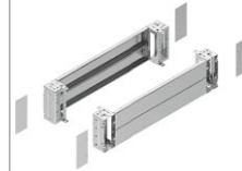
Plinth height 200 (7.87) mm (in.) (4 corners + front and back)
