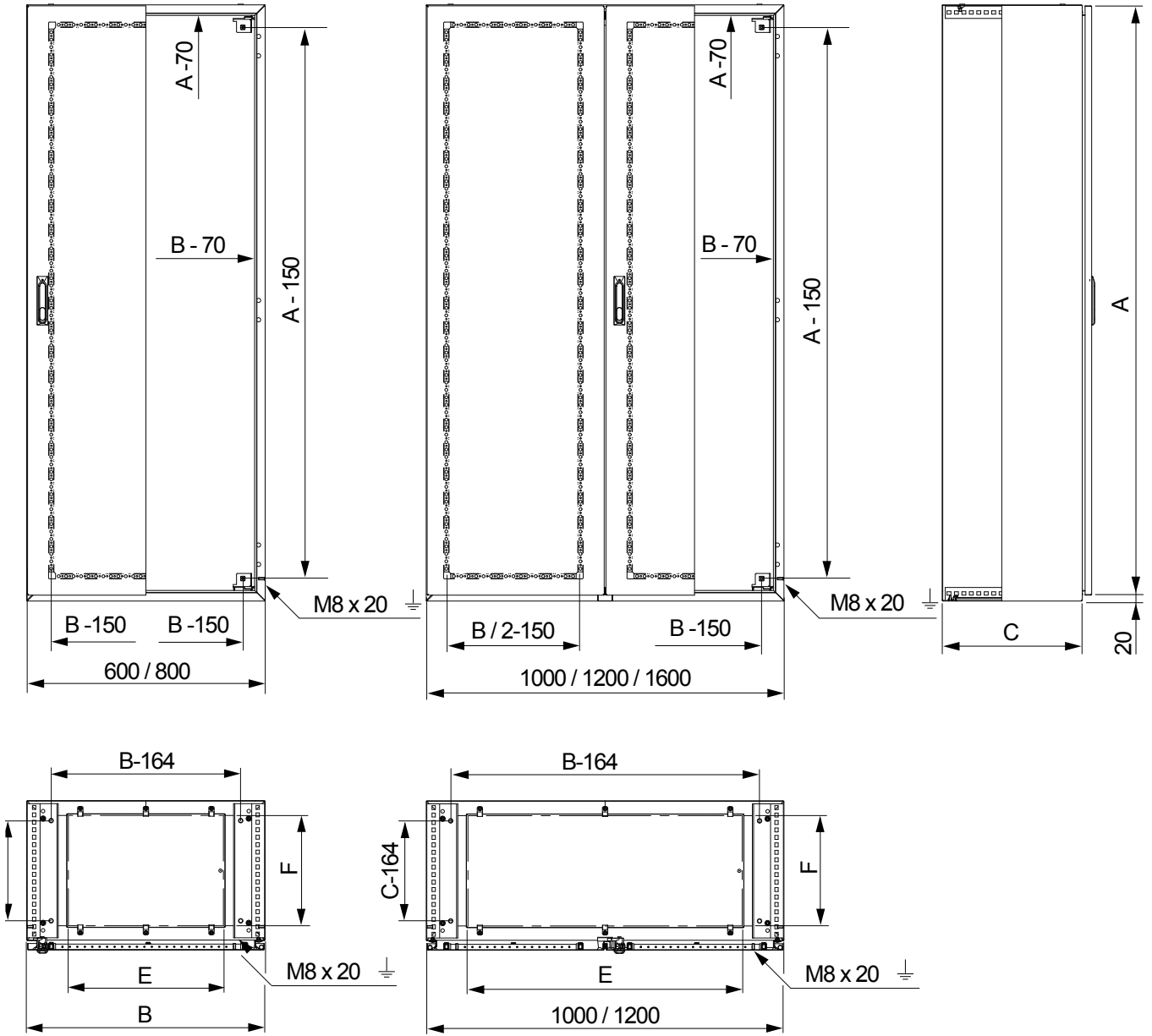
Enclosure width of 1000 (393.70) and 1200 (472.44) mm (in.)
