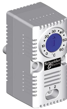
Thermostat with NO contact
