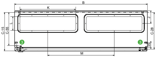
Cable entry type H: Enclosure width ≥ 800 (31.50) mm (in.).
