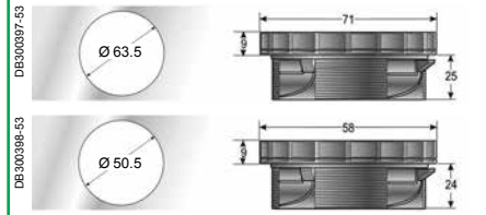
Position of the holes on the circular cable entries with diameters 50 and 63 mm
