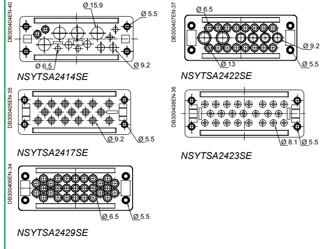
Diagrams of dimensions and positions of the holes on a rectangular cable entry
