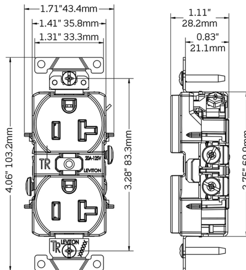
Drawing Applies to 15 & 20A Devices
