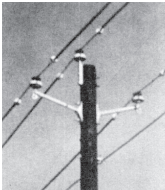
Three Phase Pole Top with APD Lightning Protectors in Place. (Only one unit is required on the load side of the line at each support for a radial circuit)
