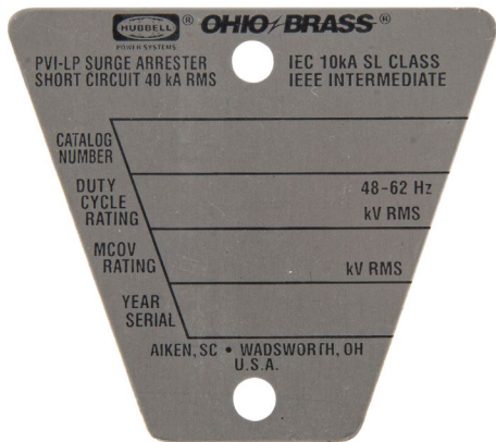
PVI-LP Nameplate
