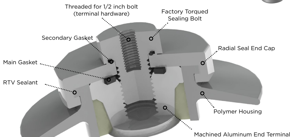
Detailed View of Sealing
