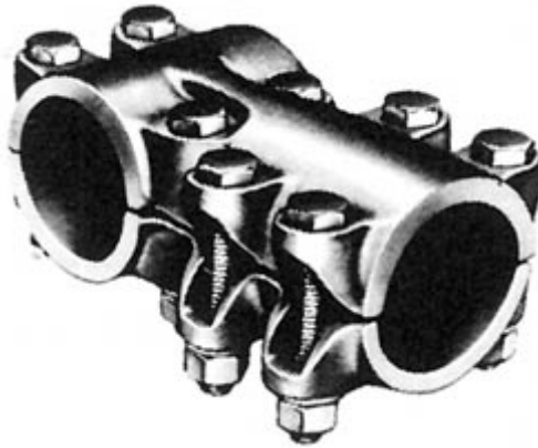
Tee, Bronze Bolted, Tube to Tube, 1-1/4 to 1 IPS/EHIPS tubes
