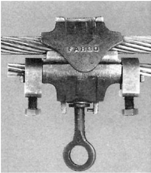
Overhead Primary Tap Connector, Hot Line Tap Connector, Aluminum, AAC|AAAC|ACSR, Range 0.502 - 0.741 in.
