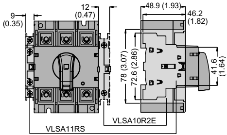
For VLS3P063R2–VLS3P125R2 Auxiliary contacts VLSA11RS VLSA10R2E
