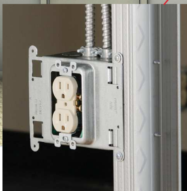
Stud-Mounted Assemblies
