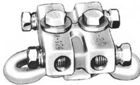
Mid Span Tap Assembly
